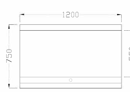
CM-120EX ■溫控開關 1200 x 750 x 300mm
