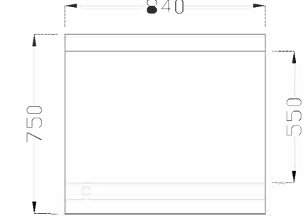
CM-84EX ■溫控開關 840 x 750 x 300mm
